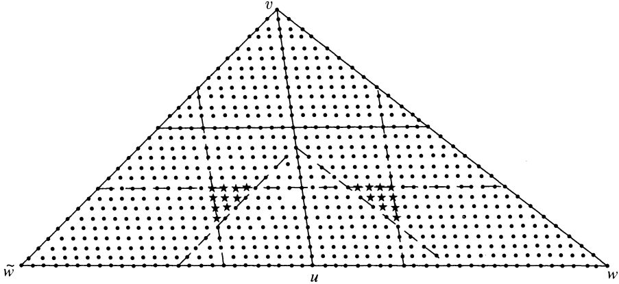
FIGURE 2. The points in X_{u,e}^n , n = \mu + 1, \dots, 2r , for a singular vertex u ( k = 26, r = 8, \mu = 12 ).
