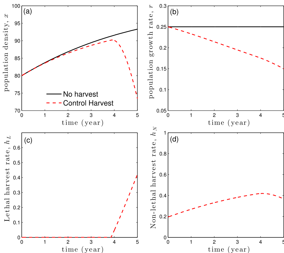
Fig. 1 Effect of optimal harvest on population density and growth rate for plants with fast growth and short lifespan. r_e = 0.25 , \tau = 5 , A = 0.1 , A_T = 0.1 , see Table 1 for other parameters
